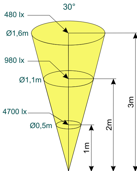
Beam angle
