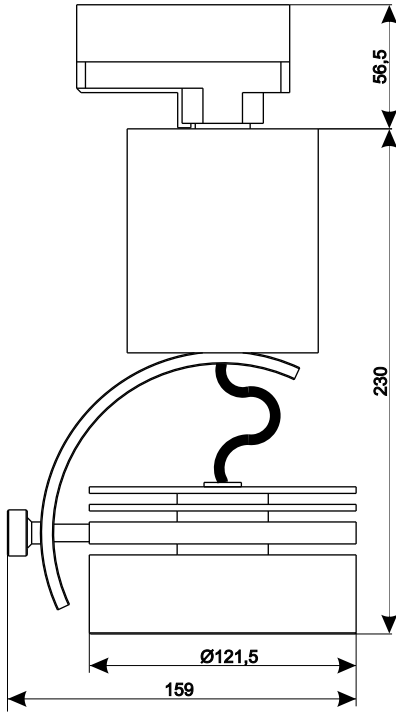
Dimensions in millimeters
