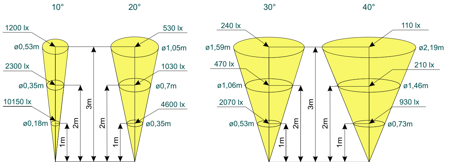
Beam angle
