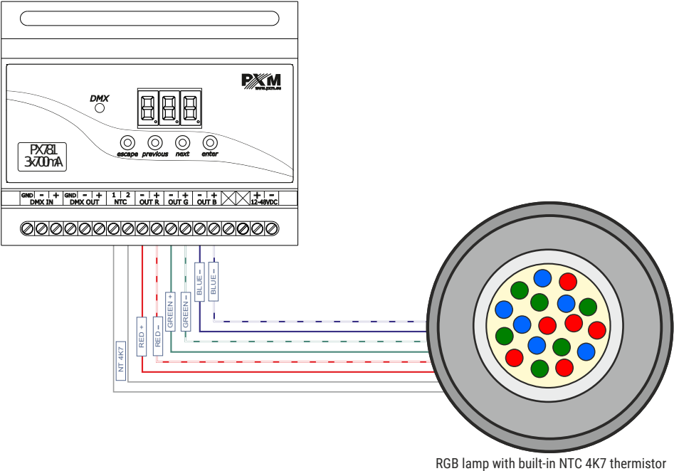
RGB lamp with built-in NTC 4K7 thermistor
